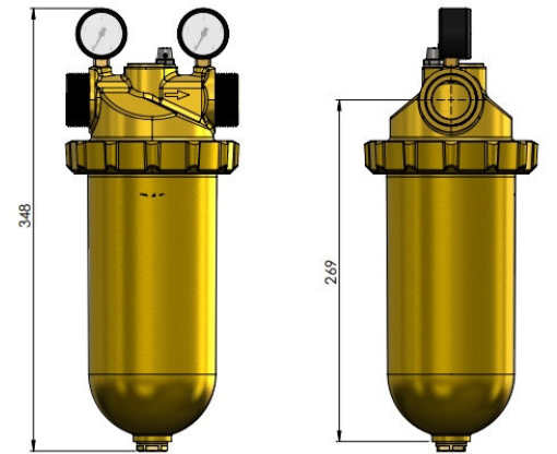
Filter 1 1/4" DN32
