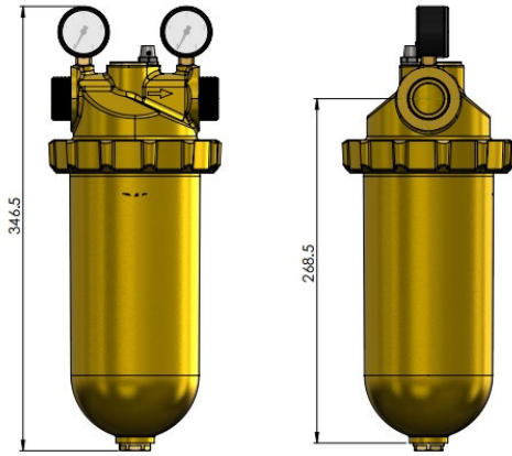
Filter 1" DN25
